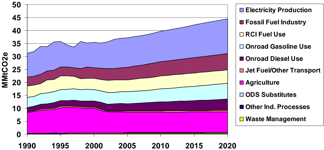
Figure 2. Montana Gross GHG Emissions by Sector, 1990-2020: Historical and Projected
