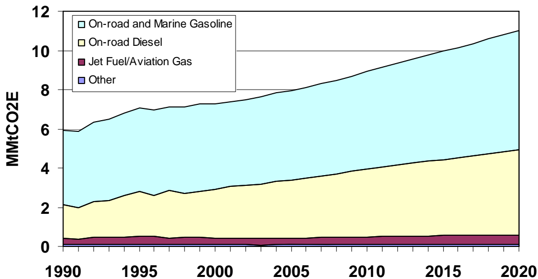
Figure C1. Transportation GHG Emissions by Fuel, 1990-2020
