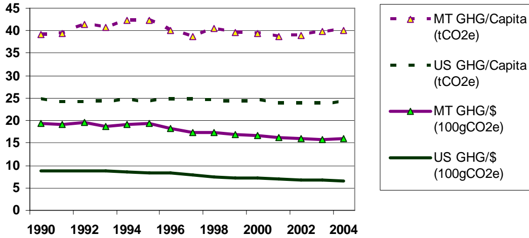
Figure 1. Historical Montana and U.S. GHG Emissions, Per Capita and Per Unit Gross Product
