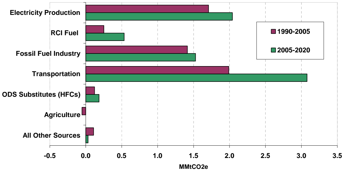
Figure 4. Sector Contributions to Emissions Growth in Montana, 1990-2020: Historic and Reference Case Projections
