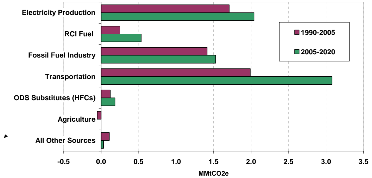
Figure 3. Sector Contributions to Emissions Growth in Montana, 1990-2020: Reference Case Projections
