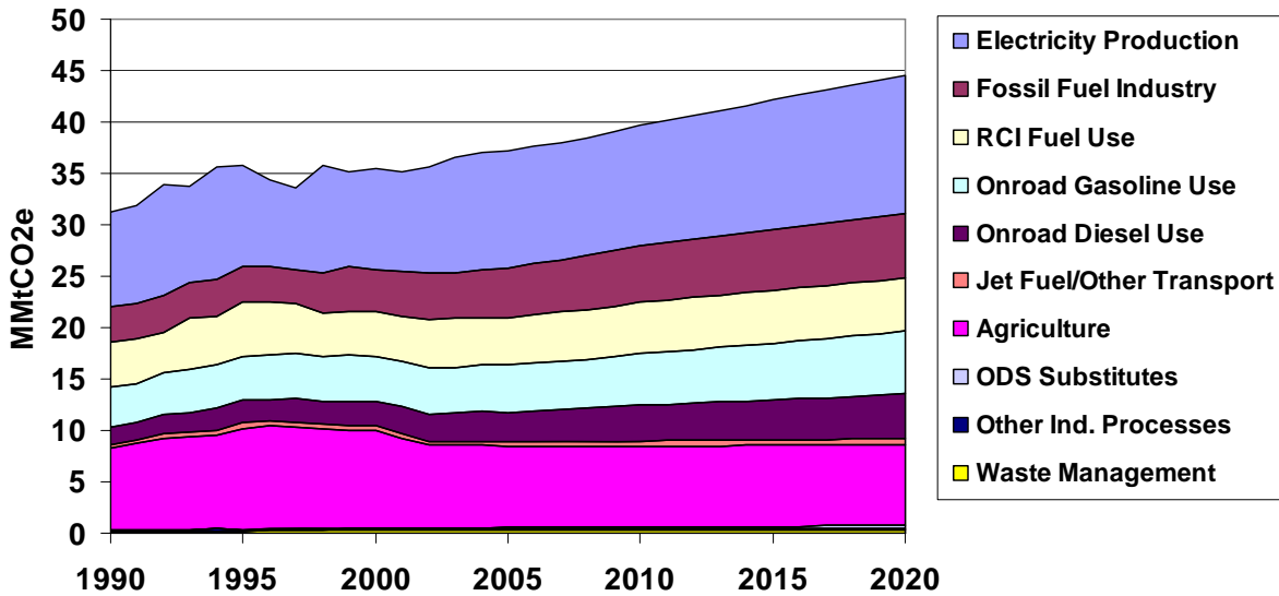
Figure 3. Montana Gross GHG Emissions by Sector, 1990-2020: Historical and Projected
