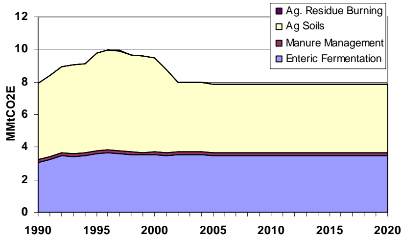
Figure F1. GHG Emissions from Agriculture
